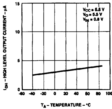
Figure 1. High Level Output Current vs. Temperature.
