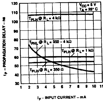
Figure 10. Propagation Delay vs. Input Current.
