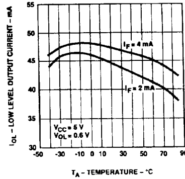
Figure 6. Low Level Output Current vs. Temperature.
