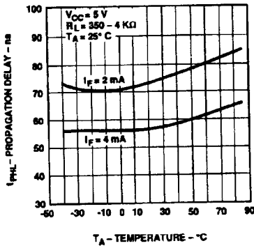
Figure 9. t_{PHL} - Propagation Delay vs. Temperature.
