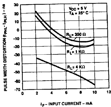
Figure 12. Pulse Width Distortion vs. Input Current.
