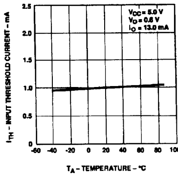
Figure 5. Input Threshold Current vs. Temperature.
