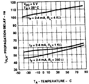
Figure 8. t_{PLH} - Propagation Delay vs. Temperature.
