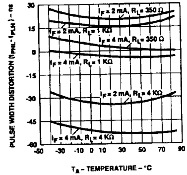
Figure 11. Pulse Width Distortion vs. Temperature.
