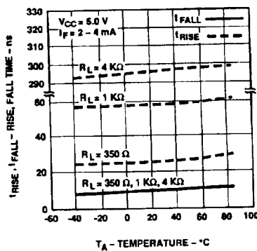
Figure 13. Rise and Fall Time vs. Temperature.
