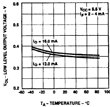
Figure 2. Low Level Output Voltage vs. Temperature.
