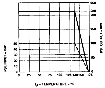
Figure 16. Dependence of Safety-Limiting Data on Ambient
