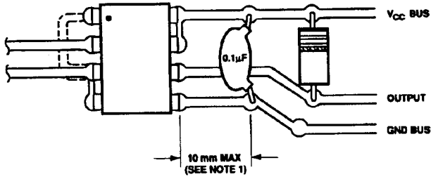
Figure 15. Recommended Printed Circuit Board Layout.
